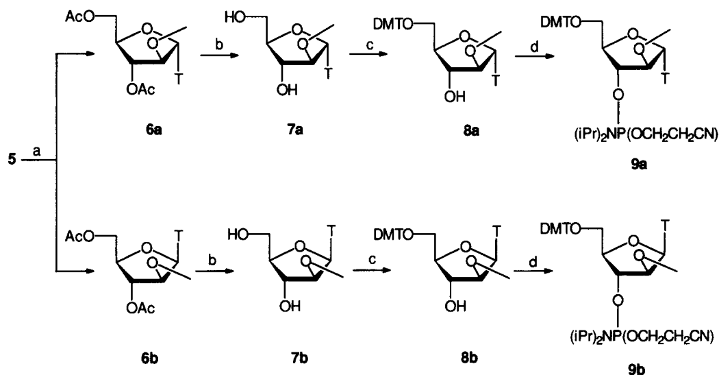
Scheme 2. (a) Silylated thymine, anhydrous 1,2-dichloroethane, TMS-triflate; (b) saturated methanolic \text{NH}_3 ; (c) DMTCl, anhydrous pyridine; (d) \text{NCCH}_2\text{CH}_2\text{OP}(\text{Cl})\text{N}(\text{iPr})_2 , anhydrous \text{CH}_2\text{Cl}_2 , N,N -diisopropylethylamine. T = thymine-1-yl; DMT = 4,4'-dimethoxytrityl.
