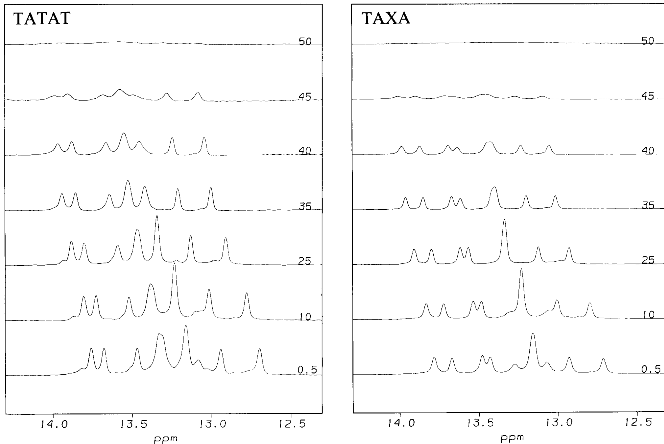
Figure 1. 1D NMR spectra of the imino-region for the duplexes DNA: G (TATAT) and DNA: H (TAXA) at different temperatures. The spectra are referenced to the spectra at 0.5 °C. The duplex concns in the samples were for G =2.0 mM and for H =1.7 mM.
